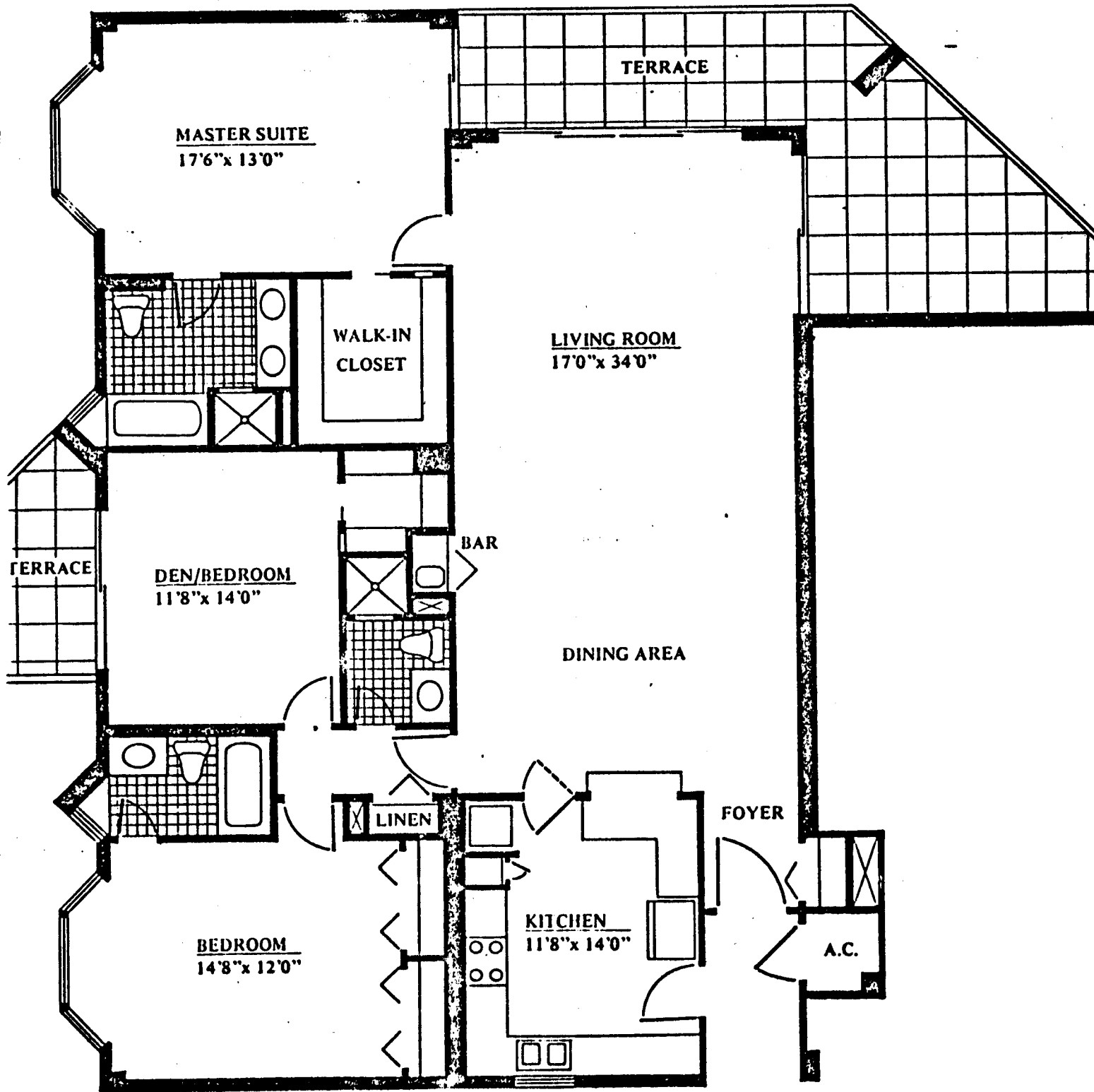
APARTMENT FLOOR PLAN "C" # 05 & 06
