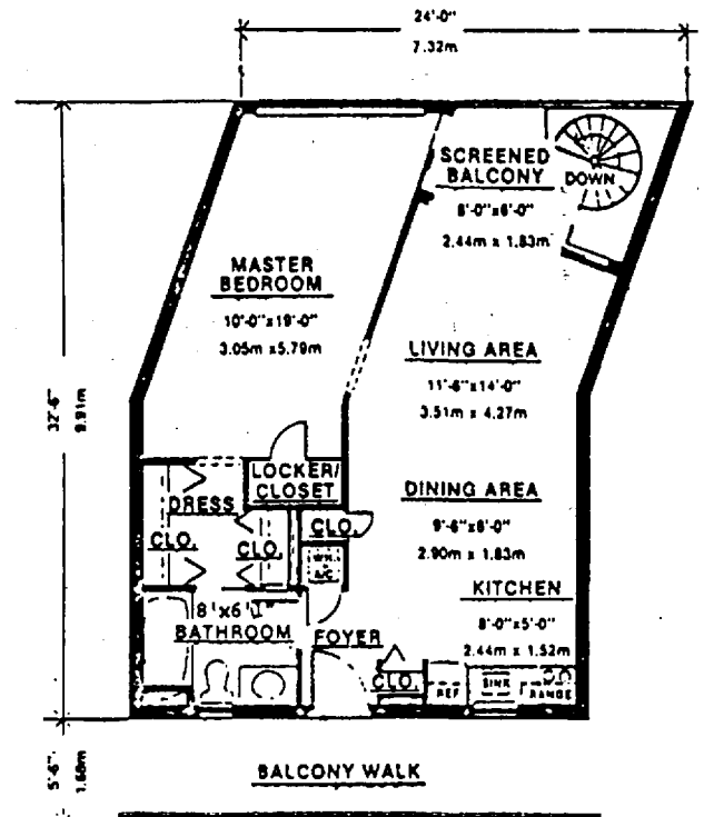
Floor Plan - Model G
