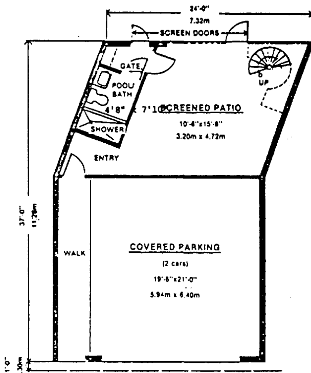
Ground Floor Plan Model G
